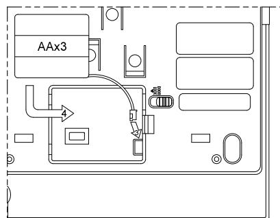
b. Install the battery
